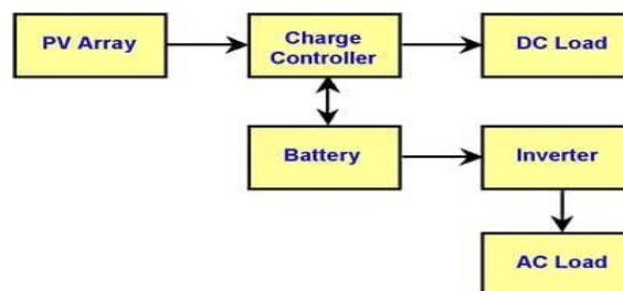
Figure: Block diagram of battery solar PV system
