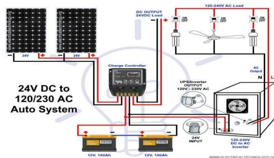
Figure: Connection diagram of battery based on solar PV system
