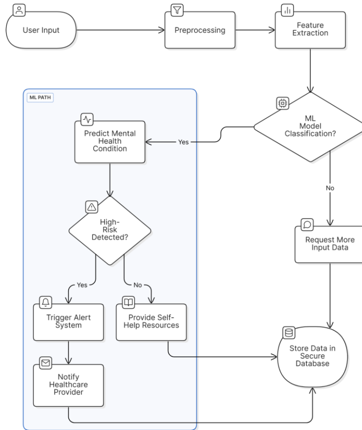
Figure 2: System architecture flowchart for mental health detection
