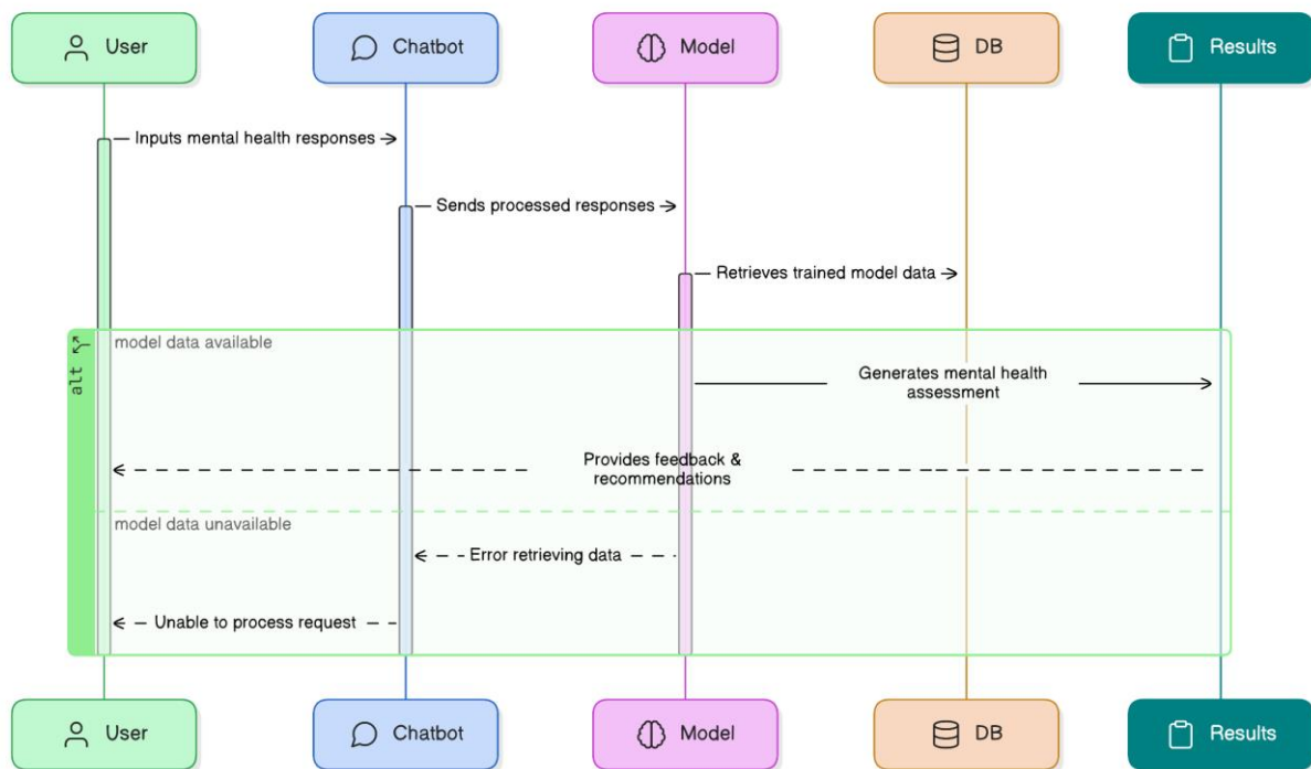
Figure 1: Dataflow in the mental health detection system
