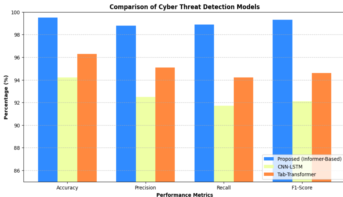
Figure 2: Comparison Graph for Existing Methods and Proposed Method
