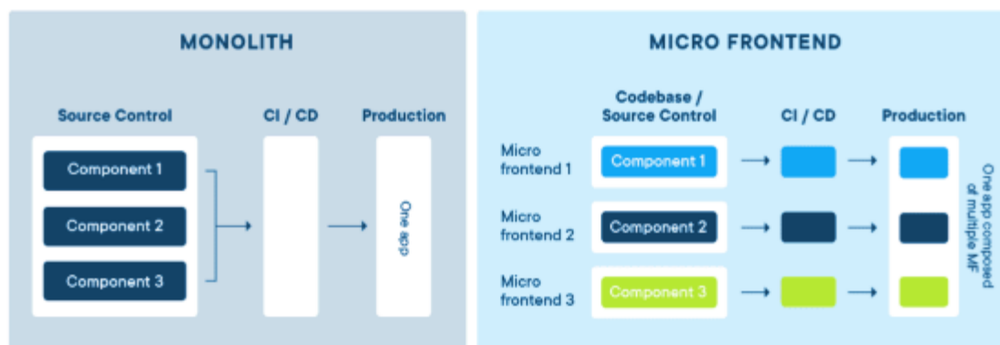
Fig. 1 Monolith vs Mirco Frontend
