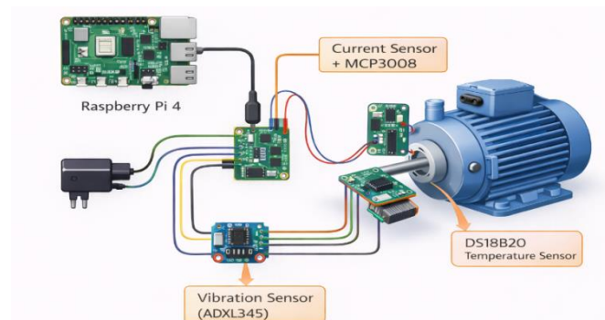
Fig. 3 hardware Implementation of proposed system
