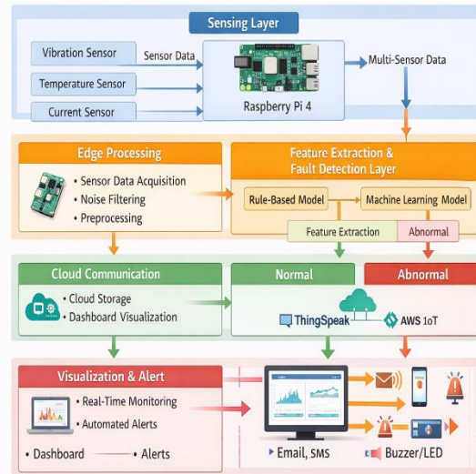
Fig.1 Proposed Architecture
