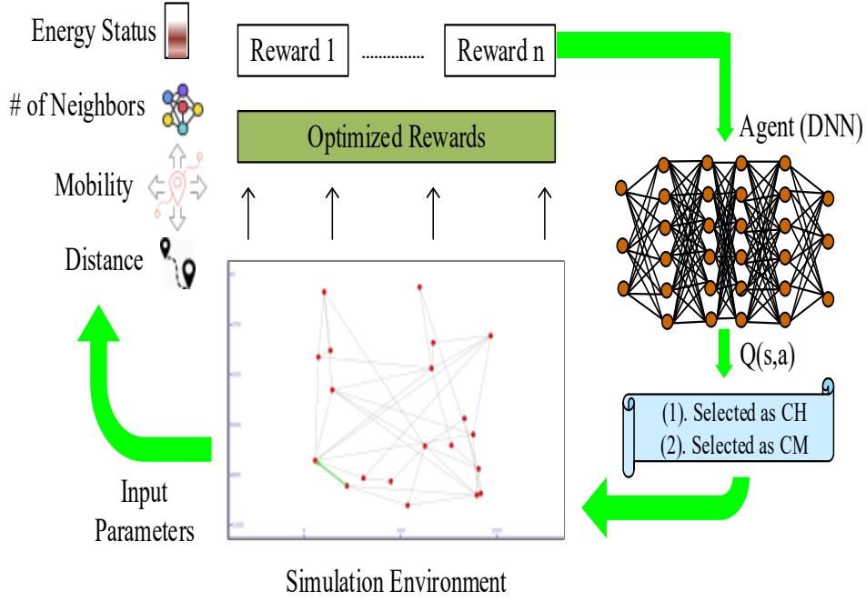
Fig.2.Flow of RoDQL algorithm
